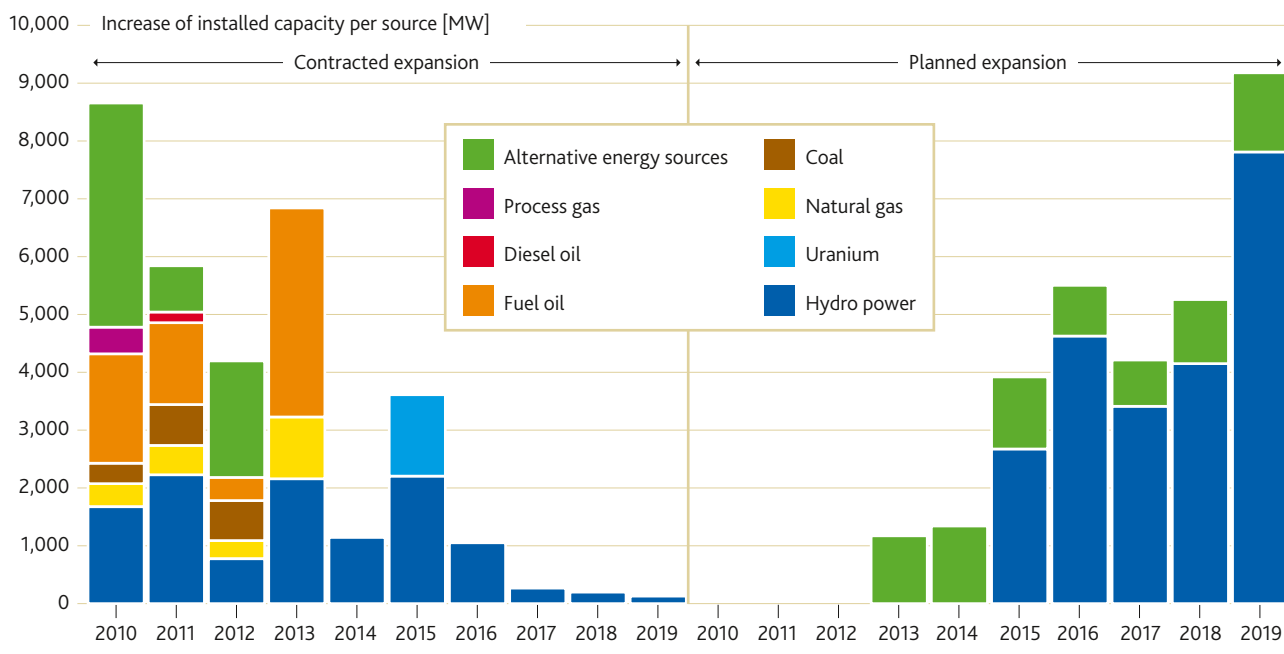
Graph 12: Expansion forecasts for technologies under Electrical Energy Ten-year Plan 2010-2019
