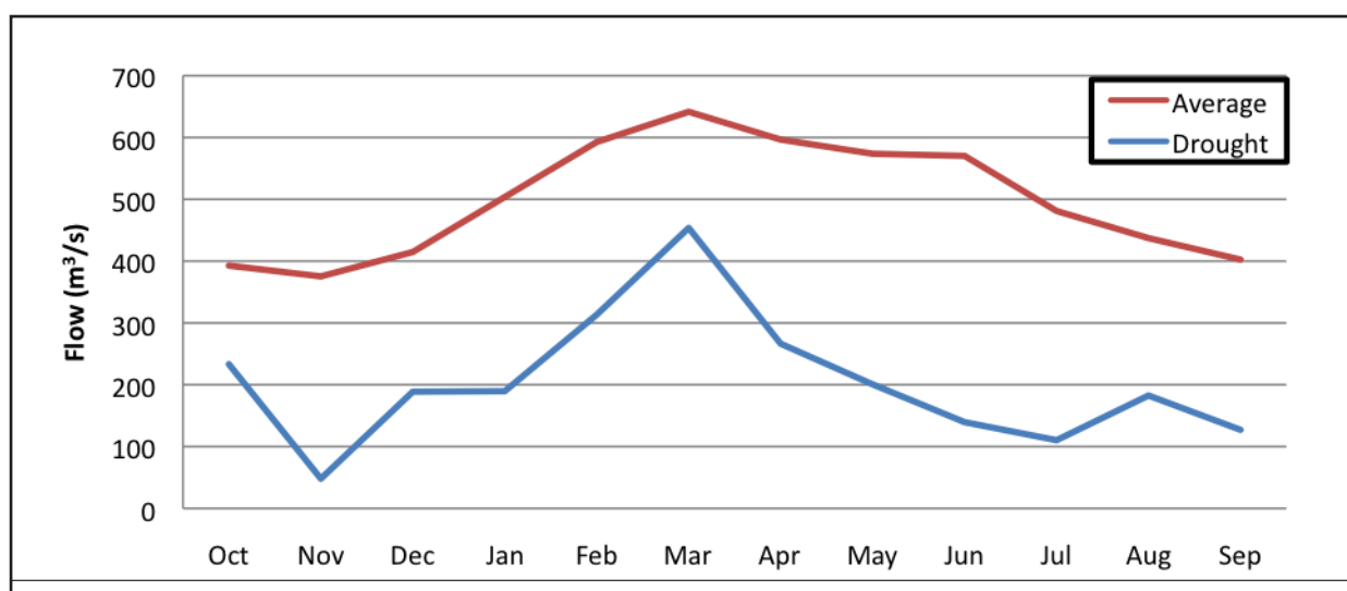
Figure A12. Mean monthly flows in the Shire/Lake Malawi sub-basin during average and drought years.
