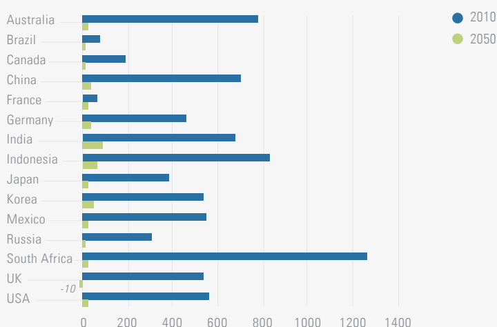
Figure 6.10. Carbon intensity of electricity production (gCO 2 /kWh)
