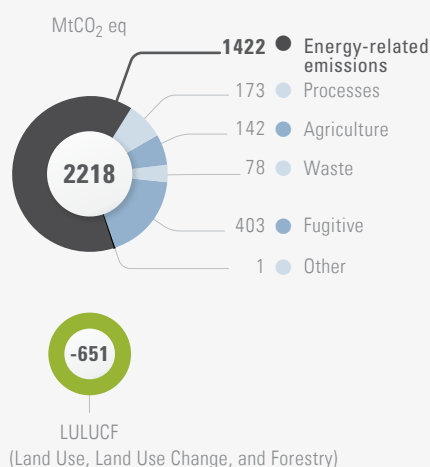
Figure 1. Decomposition of GHG and Energy CO 2 Emissions in 2010
