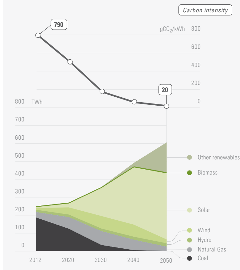
Figure 9. Energy Supply Pathway for Electricity Generation, by Source
