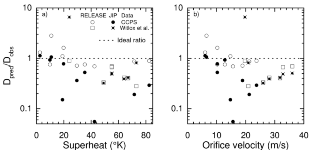
Figure 8.10: Predicted-to-observed droplet diameter ratio, D_{pred}/D_{obs} , as a function of liquid superheat and orifice velocity
