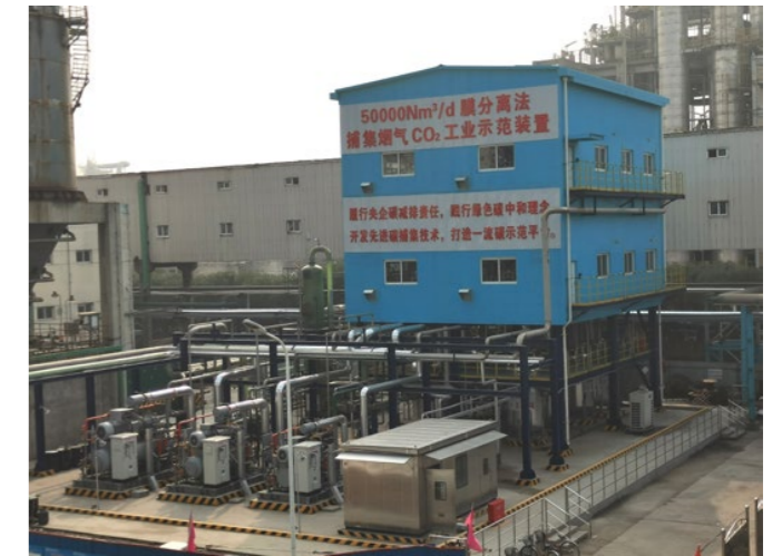
Figure 3: 50000Nm 3 /d membrane separation demonstration
