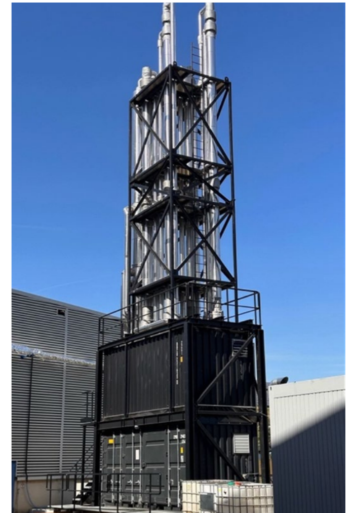
CapsolGo® unit 2 at German EfW (Energy-from-Waste) plant.
