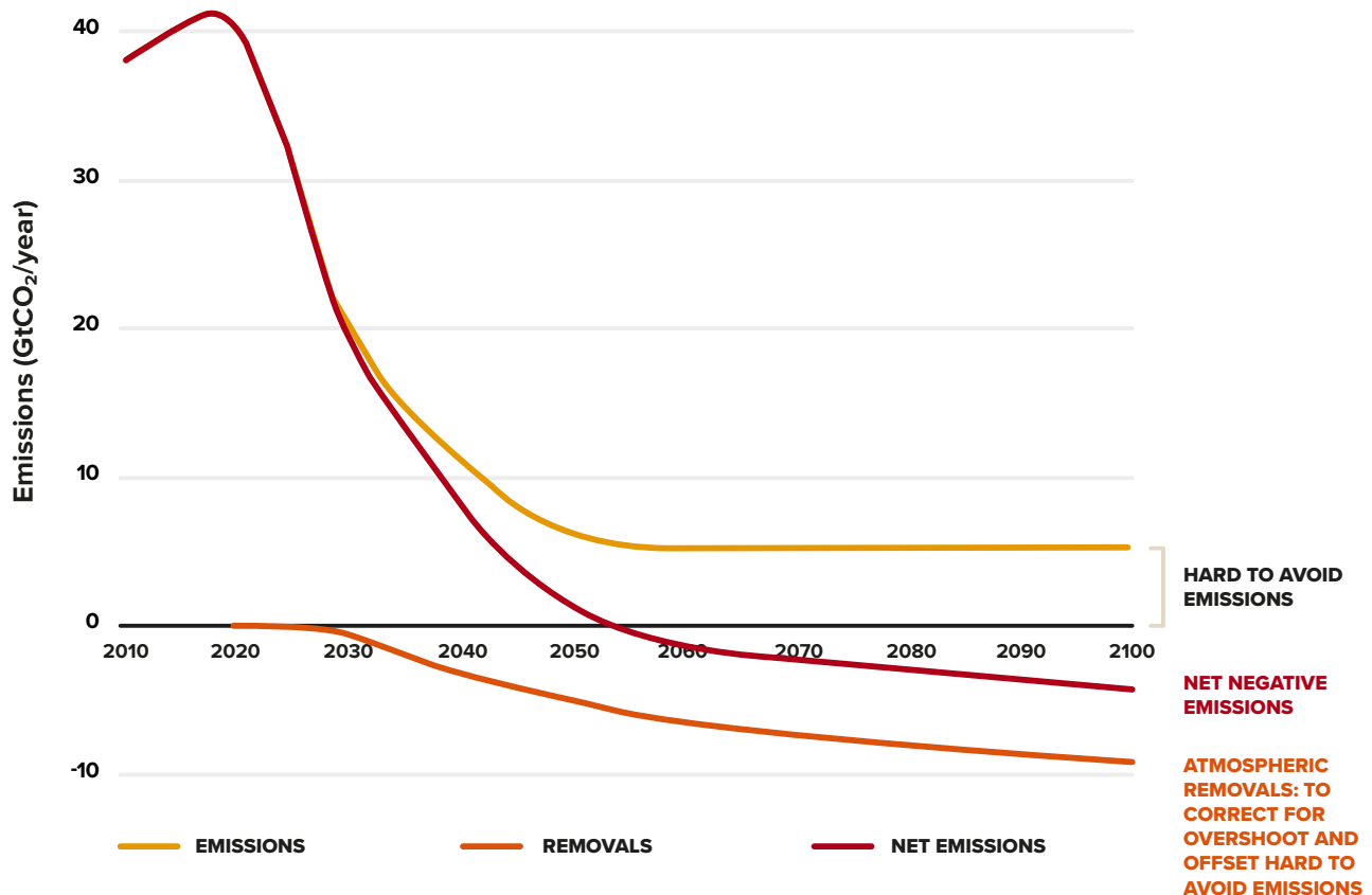
Figure 1 Illustrative Representation of Emissions Trajectory for 1.5 Celsius (Adapted from (Friedmann, Zapantis & Page 2020; Intergovernmental Panel on Climate Change (IPCC) 2018)
